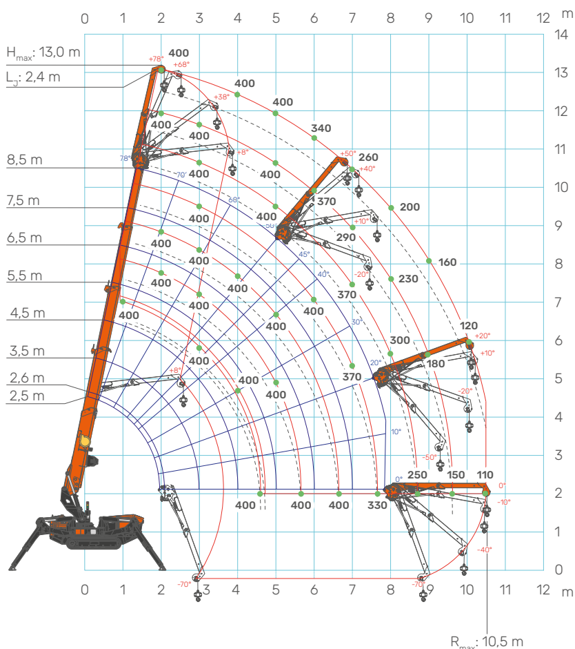
Mechanical Jib
