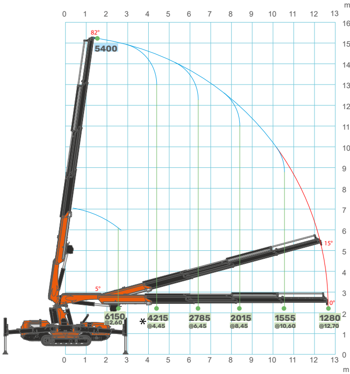
Main Boom
