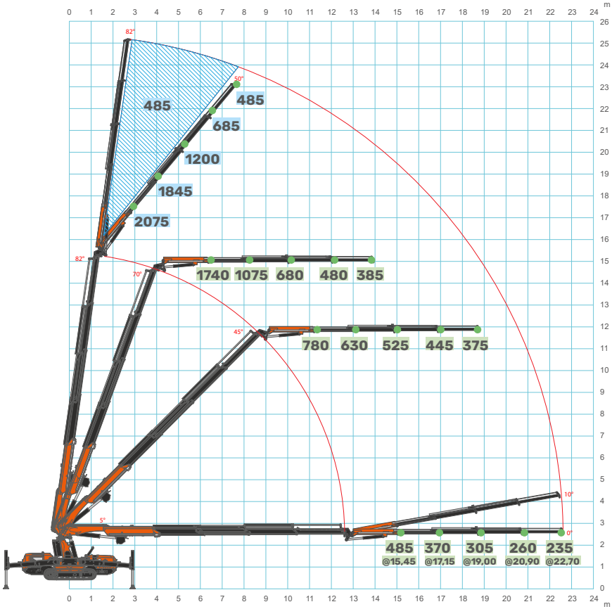
Hydraulic Jib
