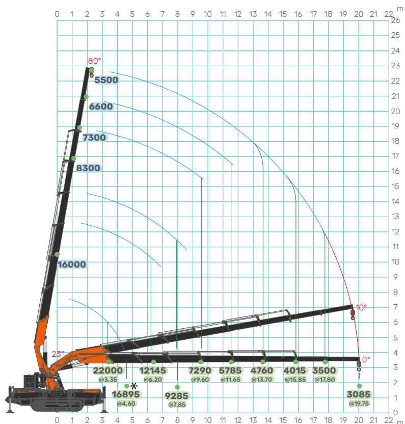
Main Boom
